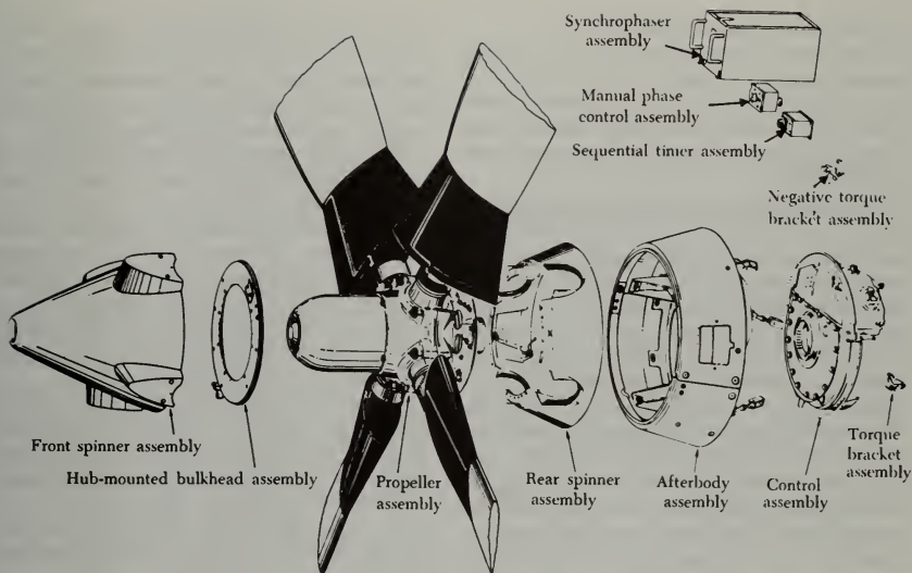
FIGURE 7-34. Propeller assembly and associated parts.
